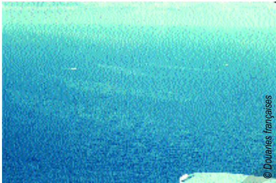
Slicks of castor oil, soya bean oil, 50/50 fuel oil and palm oil in background – aerial view. PALMOR I experiment (October 1998)
