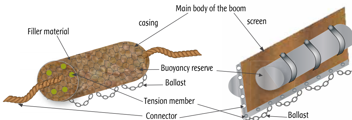
Schematic diagram showing the various components of a custom-made boom
